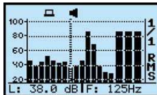
1/1 octave analysis
